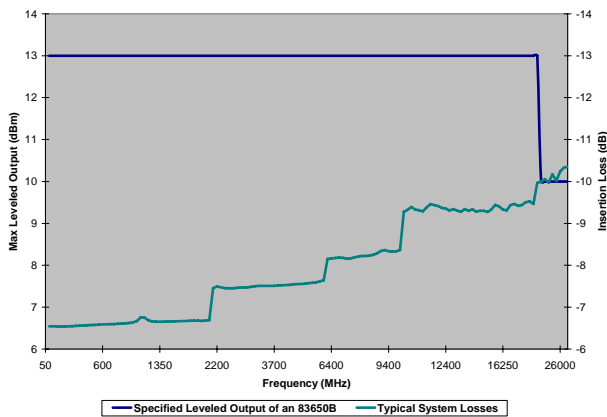
Figure 3 - Graph of signal generator specified output versus typical RF losses for 26.5 GHz System II.
