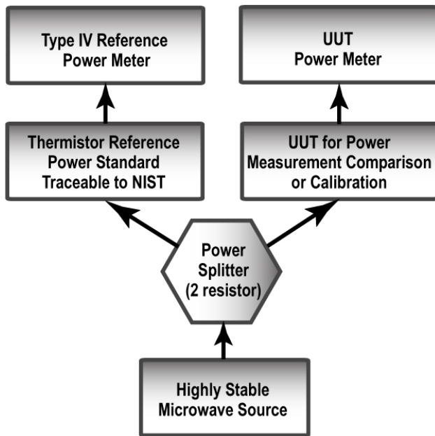
Figure 1 – Block diagram of a Direct Comparison System.
