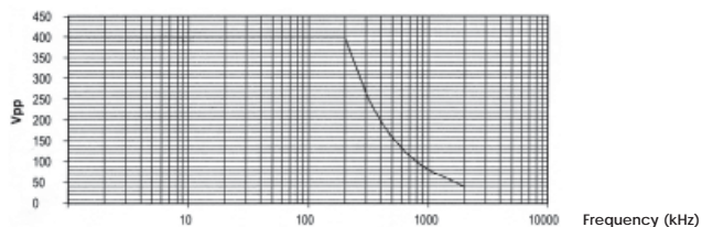
Figure 3: Maximum Vpp vs. Frequency Amplifier's maximum peak-to-peak output roll off with frequency. This is due to the amplifier's slew rate of 250 V/ \mu Sec.
