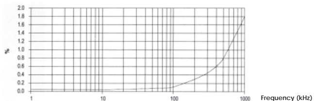
Figure 4: Distortion (Typical) Distortion measurements were made operating the amplifier at 75 % of the maximum Vpp output obtained from Figure 3.
